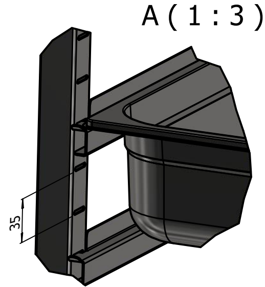
Clip in adjustable shelf runners
