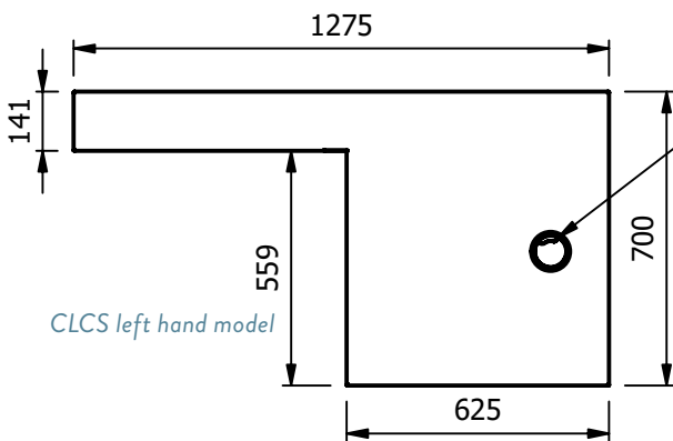
CLCS left hand model
