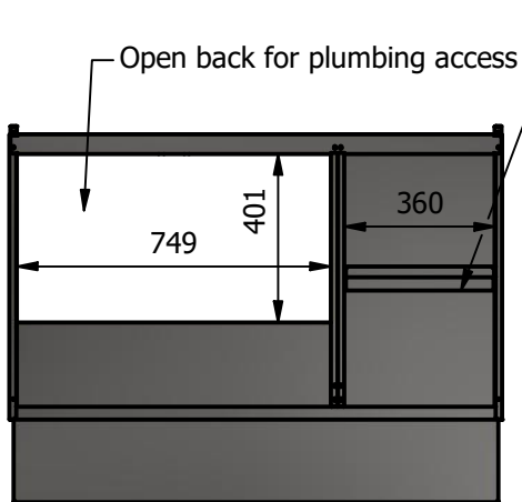
View with a standard sink top with rear up-stand and 70mm rear void
