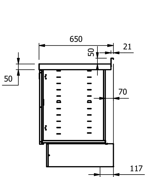
View with a standard sink top with rear up-stand and 70mm rear void
