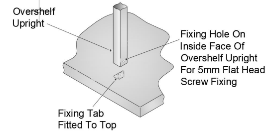
Overshelf Fixing Detail
