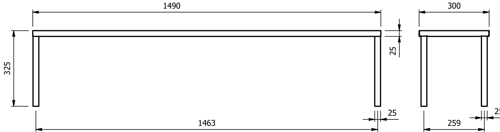
WORK TOP FIXING POINTS
