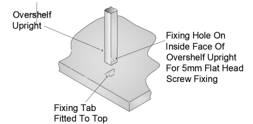
Overshelf Fixing Detail
